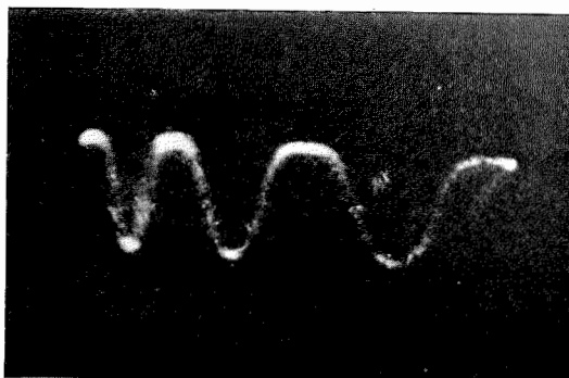
Figure 5-B—Wave-form—1500~Not Filtered
