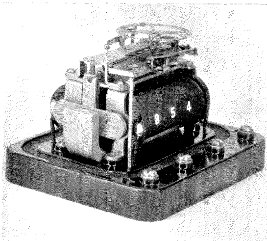
Figure 1—Telephone Train Dispatching—Selector
