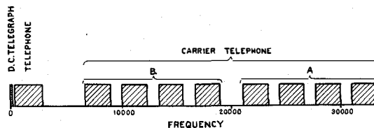
Figure 20—Assignment of Frequencies in a Representative Scheme of Carrier-Current Telephone Operation
