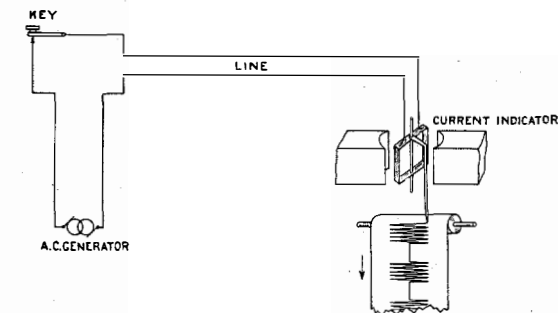
Figure 8—Diagram of an Elementary Recording Carrier-Current Telegraph Circuit Showing Signal Received Over a Line Which Has No Capacity or Inductance
