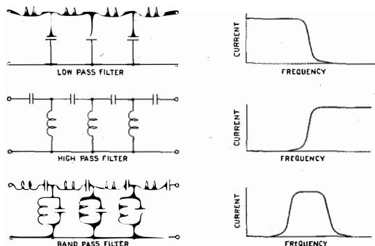
Figure 17—Typical Filter Circuits and Their Transmission Characteristics
